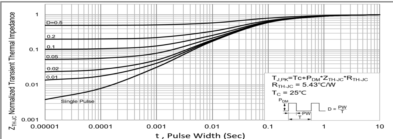
Fig.15 PJF3NA50 Normalized Transient Thermal Impedance vs. Pulse Width
