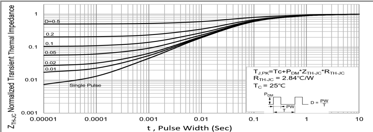
Fig.14 PJP3NA50 Normalized Transient Thermal Impedance vs. Pulse Width
